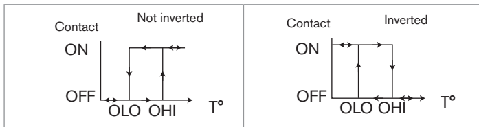
Fig. 26: Changing the output in hysteresis mode
