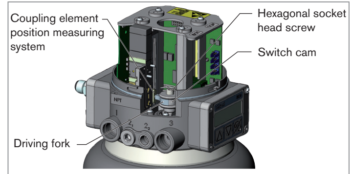
Fig. 2: Coupling position measuring system
