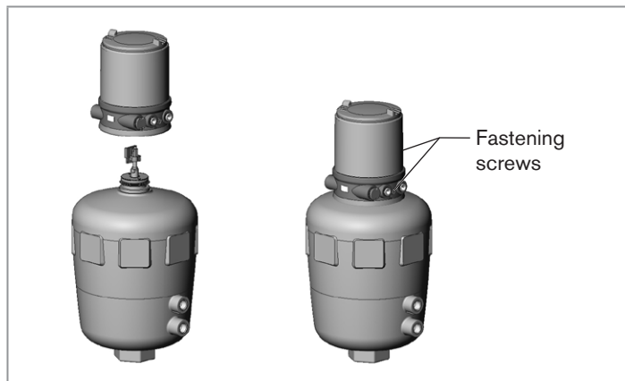
Fig. 9: Install positioner
